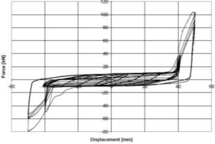
Test set-up of MADA HQ Kanada damper The first specimen complete hysteresis (force s. displacement)
